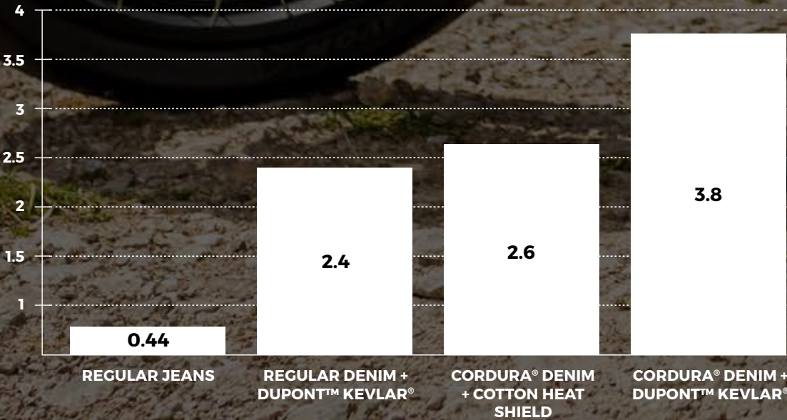
ABRASION RESISTANCE in seconds
